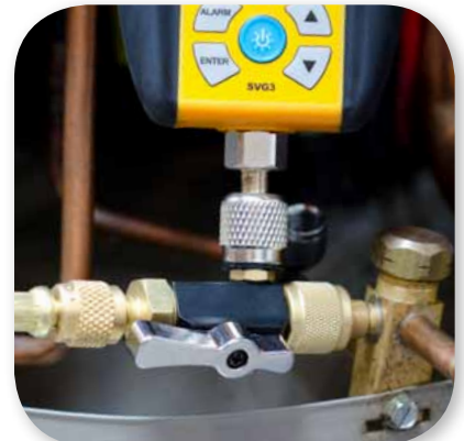
Recommended: Directly Onto Schrader Core Removal Tool
